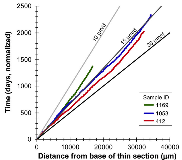
Fig. 5. Tusk growth rates calculated from second-order growth increment thicknesses for three tusk dentin slabs. Three modeled linear growth rates (10, 15, and 20 \mu\text{m}/\text{day} ) are plotted as a reference. The base of each thin section is at or near the pulp cavity or tusk axis.
