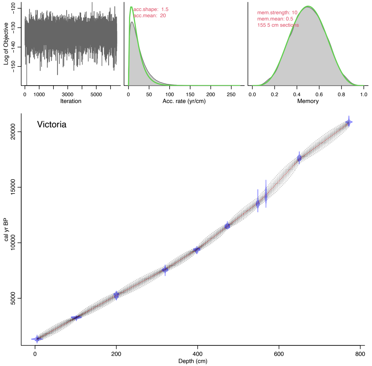
Figure S1: Updated Lake Victoria Bayesian age model using ^{14}\text{C} ages from Berke et al. (2012) and Johnson et al. (2000). Model was constructed using the 'rBacon' package (Blaauw and Christeny, 2011).
